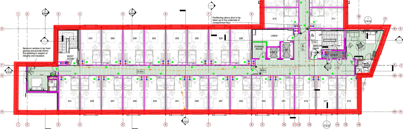
LEVEL 2 - FIRE STRATEGY PLAN Scale: 1 : 100
